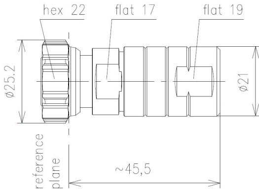
43M-SCF38-D02_Drawing
